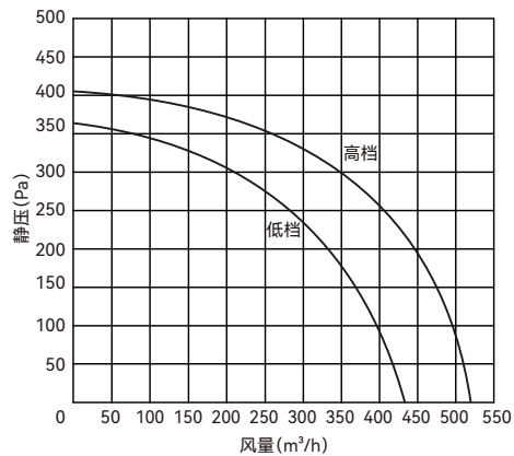
QFA-D500P(-Y) 静压-风量性能曲线
